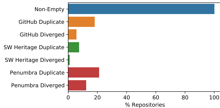
Figure 7: The Penumbra's intersection with other datasets. Of the 55343 discovered, non-empty repositories, 18% have a first commit hash that can also be found on GitHub (GitHub Duplicate), but 30% of those repositories diverge and contain code not found on GitHub (GitHub Diverged). Likewise, 7% of Penumbra repositories have a first commit archived by Software Heritage [1], and 14% of those contain code not archived by Software Heritage. Finally, 21% of Penumbra repositories share a commit with one or more other Penumbra repositories, and of these, 58% have unique final commits.
