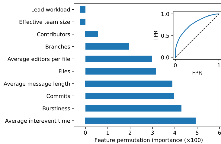
Figure 6: Random forest model to delineate Penumbra and GitHub samples. Feature permutation importance (Sec. 2.5) once nonlinear random forest regressions were trained to predict whether a project was on GitHub or in the Penumbra. The predictive performance is shown in the inset using an ROC curve of true positive rate (TPR) and false positive rate (FPR).
